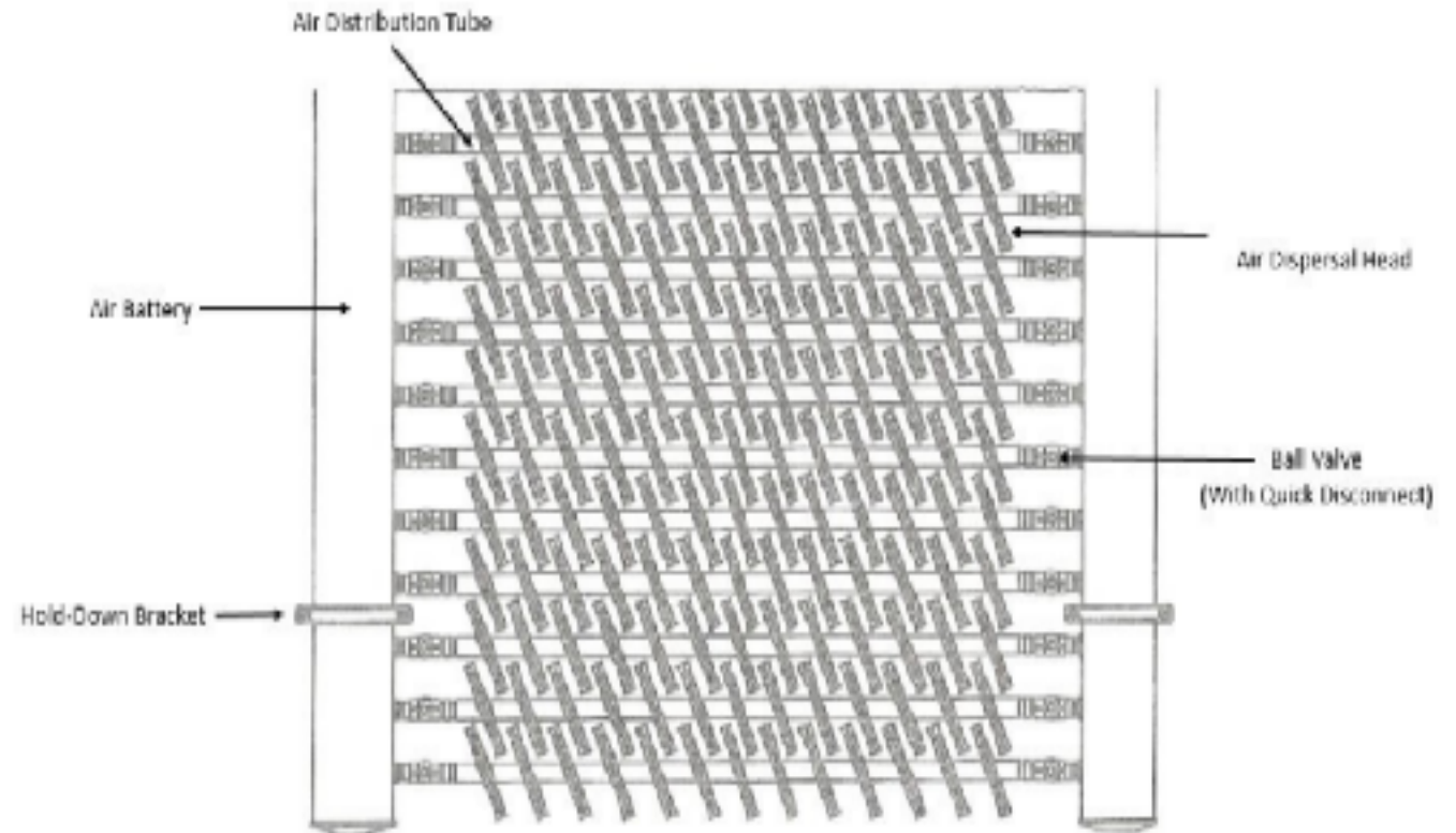
TYPICAL AIR BATTERY
